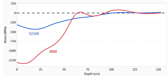
Fig. 23. Effect of material chemistry on residual stress.
